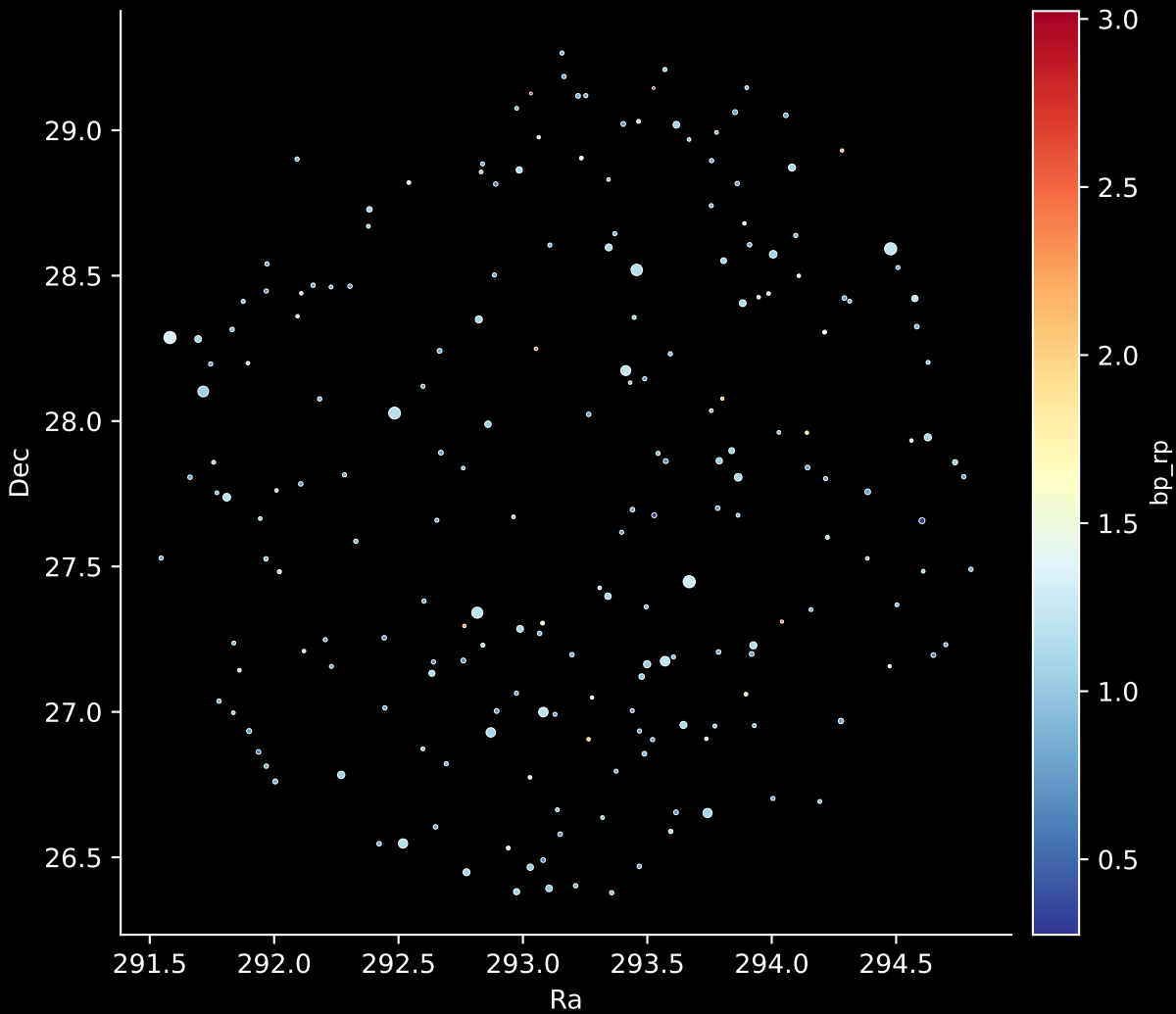
APOGEE DR17 Field: [101+89_MGA] Stars: 206
