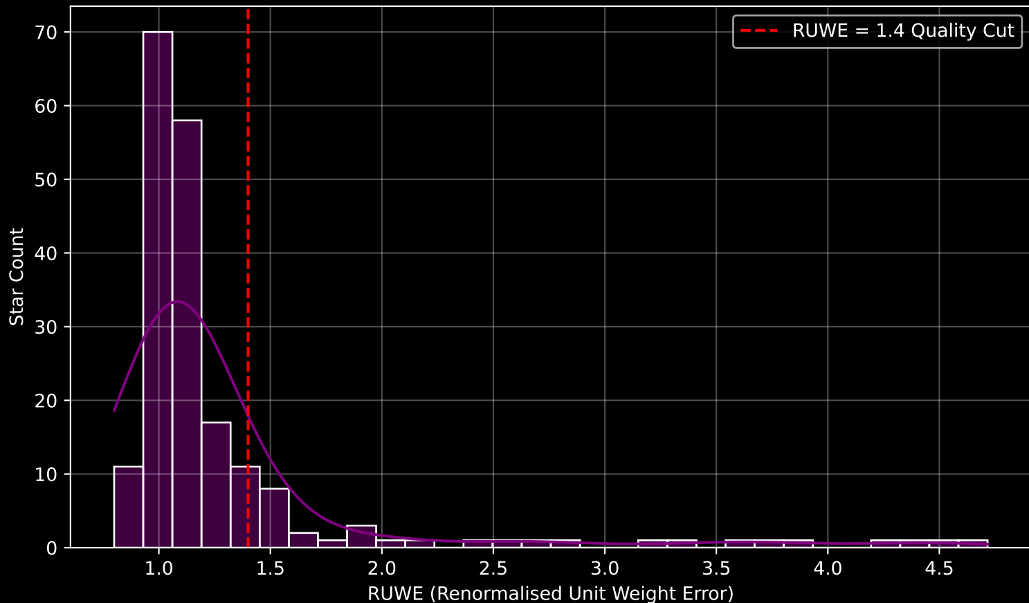
GAPOGEE DR17 Field [101+89_MGA] RUWE Distribution (n= 196)
