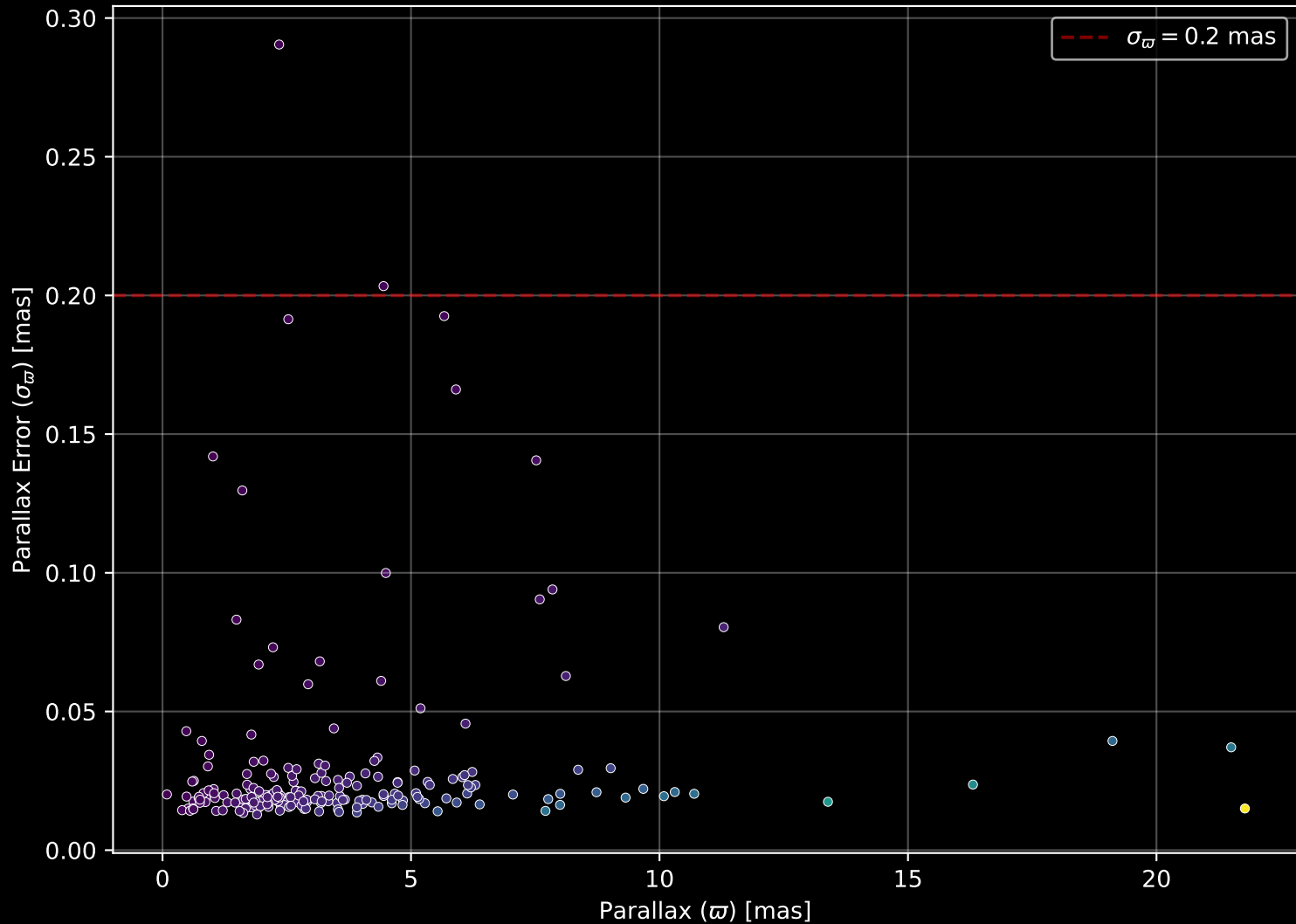
APOGEE DR17 Field: [101+89_MGA] Parallax Quality (n= 206)
