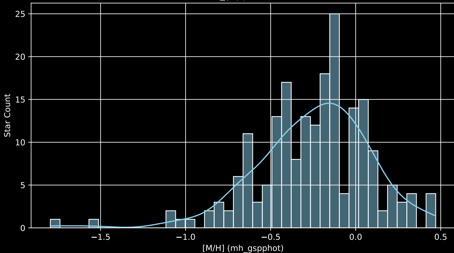
APOGEE DR17 Field: [101+89_MGA [M/H] (mh_gspphot) (n= 204)
