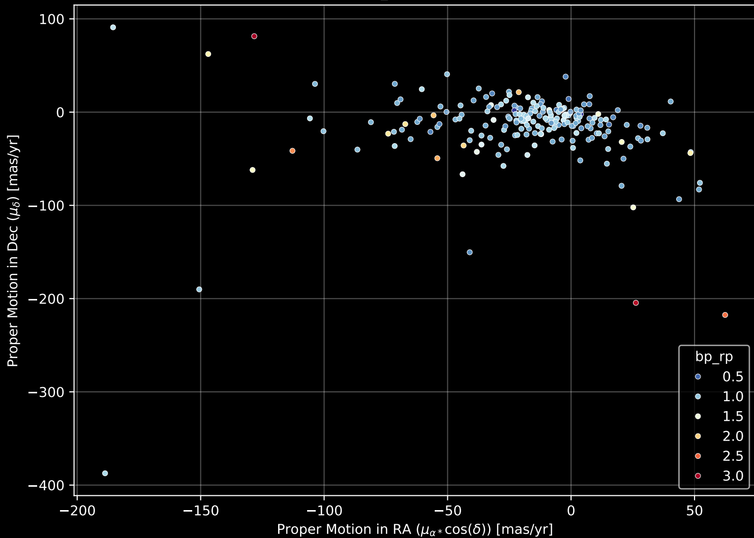
APOGEE DR17 Field: [101+89_MGA] Proper Motion Diagram (n= 206)
