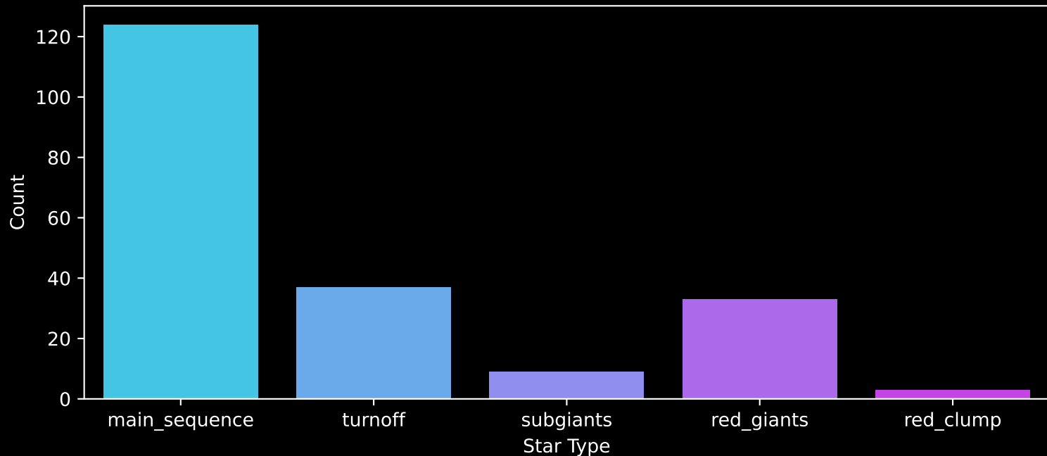
APOGEE DR17 Field: [101+89_MGA] Count plot of Star Type
